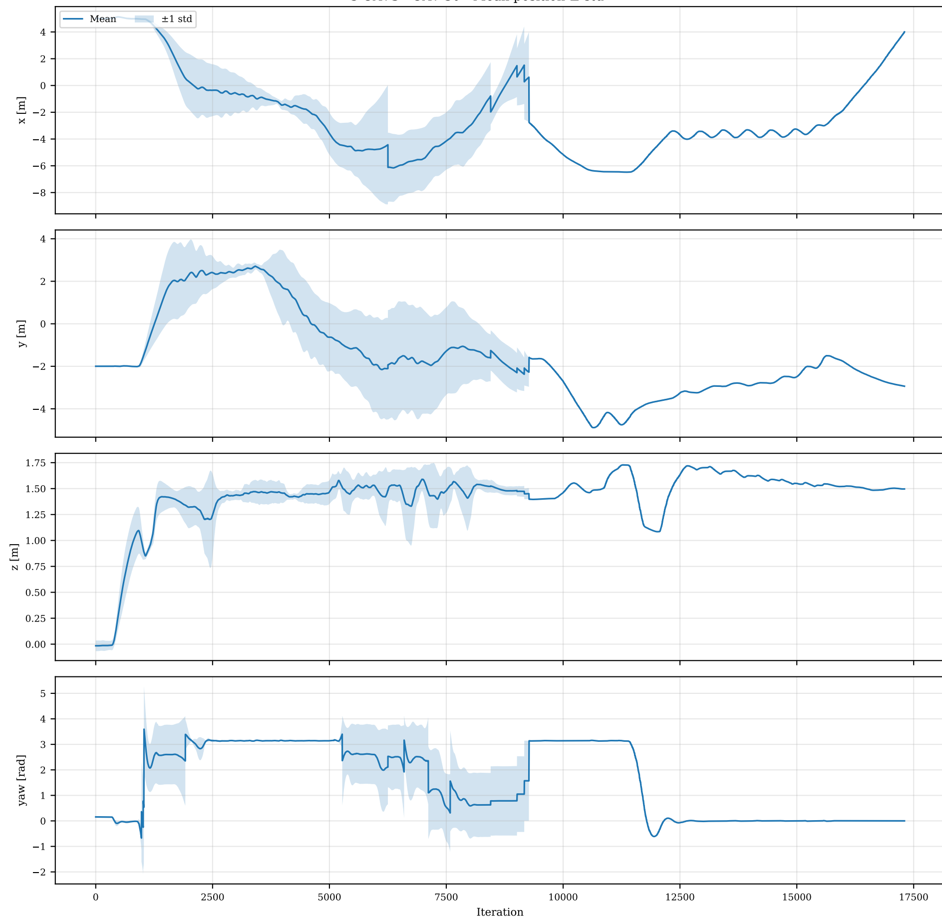
3 UAVS - UAV 30 - Mean position \pm std
